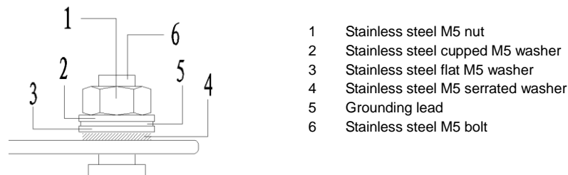
Figure-1 Grounding panel frame with stainless steel grounding & bonding equipment
