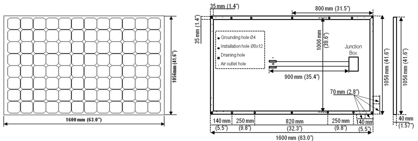
Figure-3 Dimension of Module, and Position of Mounting Holes, GS-S- nnn -Fab8, “ nnn ” is from 240 to 250
